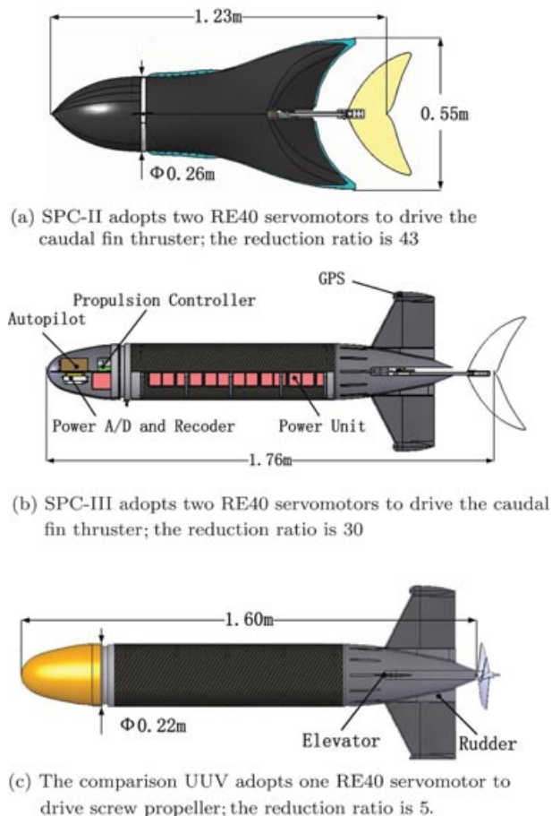
Figure 1. SPC-II and SPC-III robotic fish and the comparison UUV.
