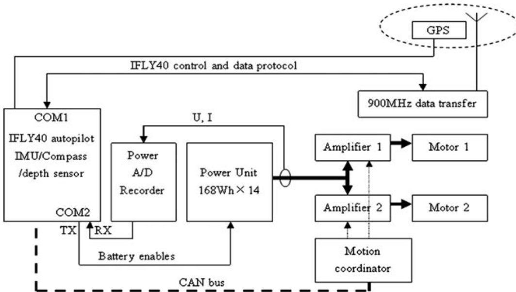
Figure 6. Electrical system of SPC-III robotic fish.
