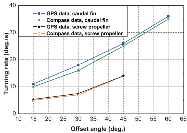
Figure 12. Turning rates of SPC-III and the comparison AUV, with translational speed of about 1.1 m/s.
