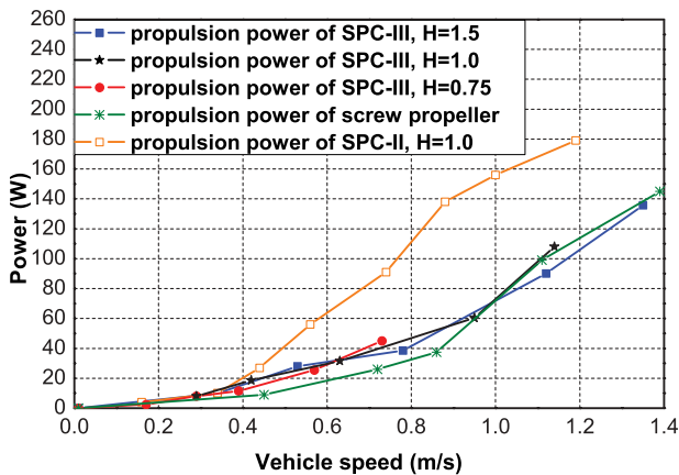
Figure 10. Propulsion power of SPC-III, SPC-II, and screw propeller at different swimming speeds.
