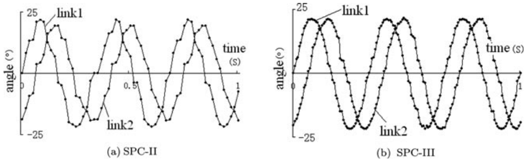
Figure 5. Flapping profiles of SPC-II and SPC-III robotic fish.
