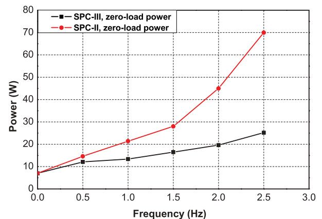
Figure 2. Zero-load powers of SPC-II and SPC-III robotic fish.
