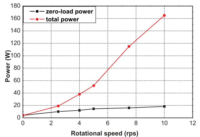
Figure 9. Zero-load and total power of screw propeller.
