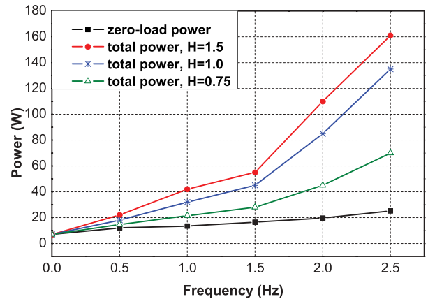
Figure 8. Zero-load and total power of caudal fin.
