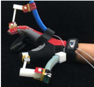
Fig.5. The two-fingered glove using soft actuators.
