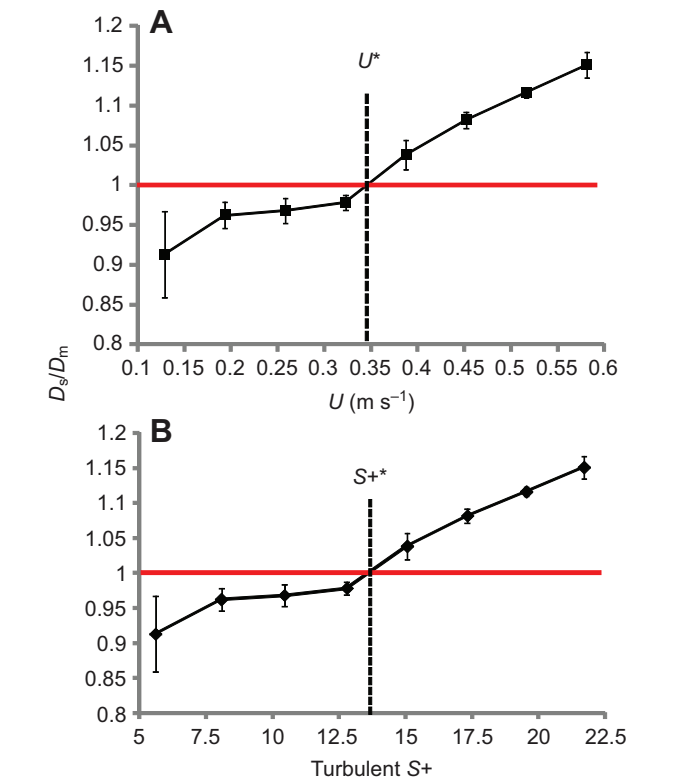
Fig. 2. Drag force ratio dependence on flow speed and dimensionless denticle ridge spacing for turbulent flows. D_s/D_m is the ratio of static drag of the smooth foil ( D_s ) to static drag of the shark skin foil ( D_m ). (A) Dependence on the flow speed ( U ). (B) Dependence on dimensionless denticle ridge spacing for turbulent flows (turbulent S+). The red solid lines represent D_s/D_m=1 , which indicates that the synthetic shark skin foil has the same static drag force as the smooth foil. The vertical dashed lines in A and B indicate ‘critical’ flow speed ( U^* ) and critical S+ ( S+^* ), respectively, where drag of the shark skin membrane is greater than that of the smooth control. Drag forces are means from N =5 trials for each measurement, which lasted 20 s. Error bars are ±1 s.e.m., and are the same for A and B. For further explanation, refer to the Materials and methods. Drag force values for the shark skin and smooth control membranes are provided in Table 1.
